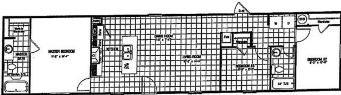
15 x 72' The Bronze Three Bedroom, Two Bath - 1080 Sq. Ft.
